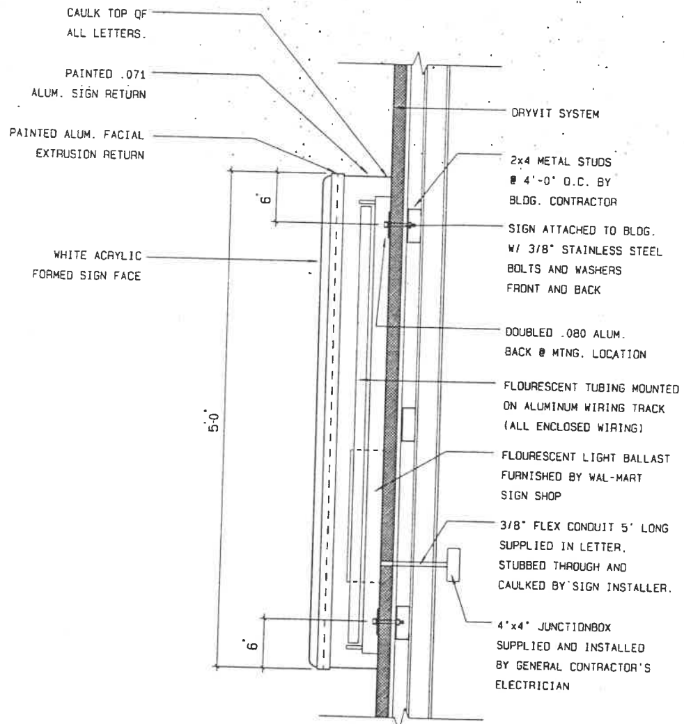
1 5'-0" SIGNAGE SECTION
