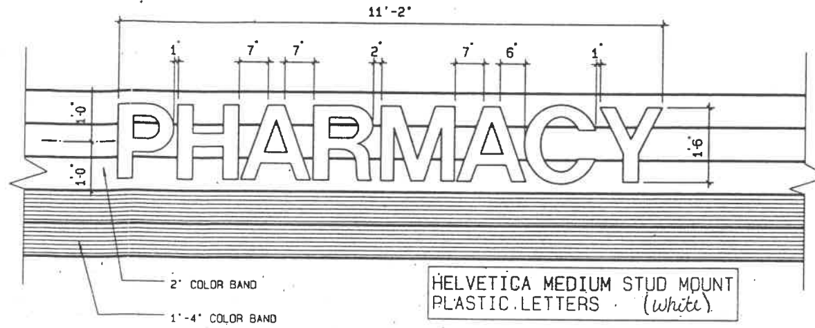
2 18' PHARMACY SIGN 15.75 • NOT TO SCALE - PATTERN PROVIDED 36 STUDS
