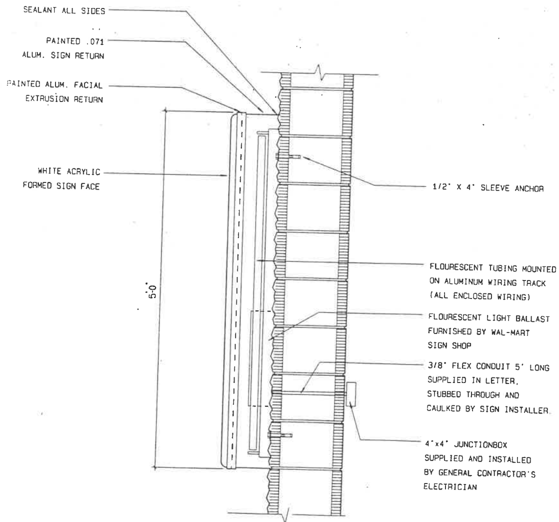
5'-0" SIGNAGE SECTION ON SPLITFACE
